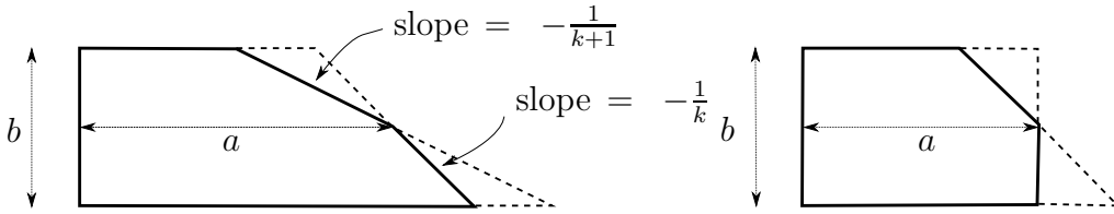
FIGURE 4. H'_{a,b,k} for k \geq 1 and H'_{a,b,0} .
