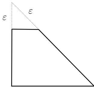
FIGURE 1. A corner chopping of size \varepsilon .
