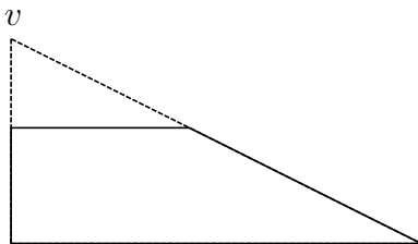
FIGURE 5. The vertex v is not smooth.
