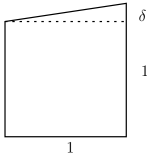
FIGURE 6. The polygon Q_\delta .
