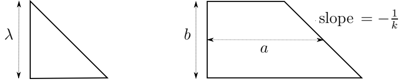
FIGURE 2. The Delzant triangle \Delta_\lambda and the Hirzebruch trapezoid H_{a,b,k} .
