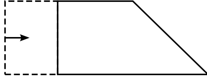
FIGURE 3. Moving an edge parallel to itself.
