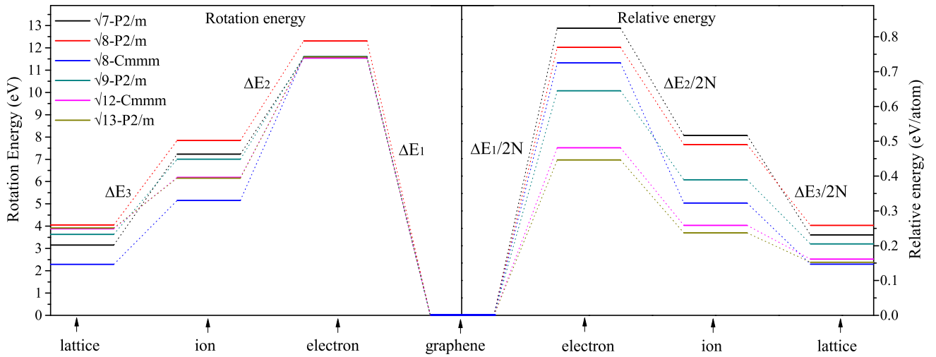
FIG. 5: Energy splitting and inversion model (left: rotation energies eV per cell; right: relative energies eV/atom relative to graphene) based on the comparison of energy changes between \sqrt{7} , \sqrt{8} - Cmmm , \sqrt{8} - P2/m , \sqrt{9} , \sqrt{12} and \sqrt{13} in three steps after bond-rotation, namely, electronic minimization in fixed configuration (electron), ionic relaxation (ion), as well as full lattice and ionic relaxation (lattice).
