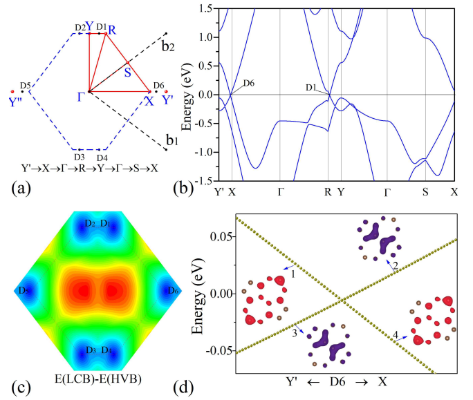
FIG. 2: The first Brillouin zone (BZ) (a), the band structures (b), the 2D color mapping of the energy differences between LCB and HVB (c), as well as the band decomposed charge density distributions of SW-graphene (d).
