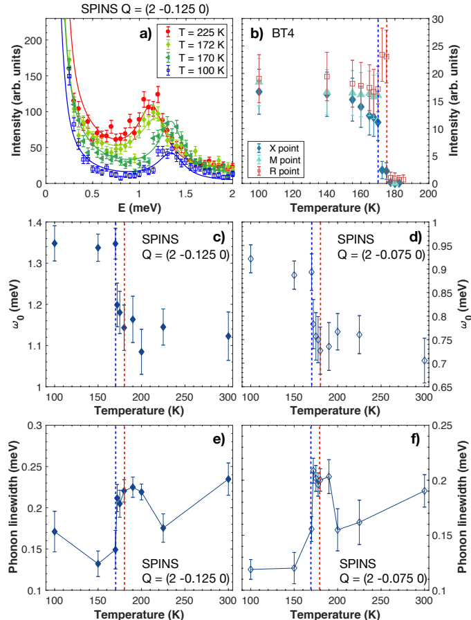
FIG. 3. (a) Constant Q = (2 -0.125 0) scans at several temperatures, measured on SPINS (NIST). (b) Temperature evolution of the integrated intensity measured with E = 0 at the X , M and R points, measured on BT4 (NIST). (c) - (d) Temperature evolution of the energy position of the TA 1 mode, extracted at the Q = (2 -0.125 0) and Q = (2 -0.075 0) positions, respectively. (e)-(f) Temperature evolution of the TA 1 phonon linewidth, extracted at the Q = (2 -0.125 0) and Q = (2 -0.075 0) positions, respectively.
