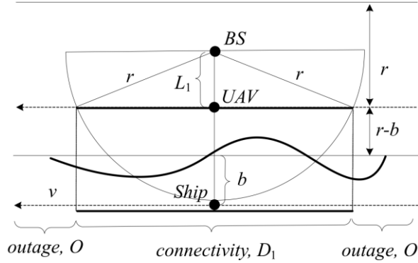
Figure 24. Connectivity model for UAV Base station
