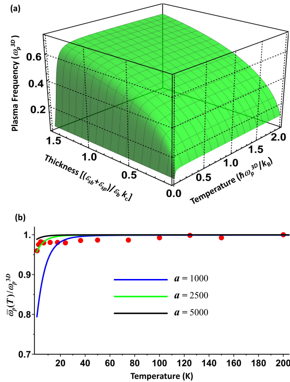
Fig. 5. (a) Plasma frequency general behavior as a function of dimensionless temperature and film thickness as computed from Eq. (5). (b) Analysis of the plasma frequency temperature dependence using the confinement induced nonlocal dielectric response model of the finite-thickness plasmonic film [24]. See text for details.
