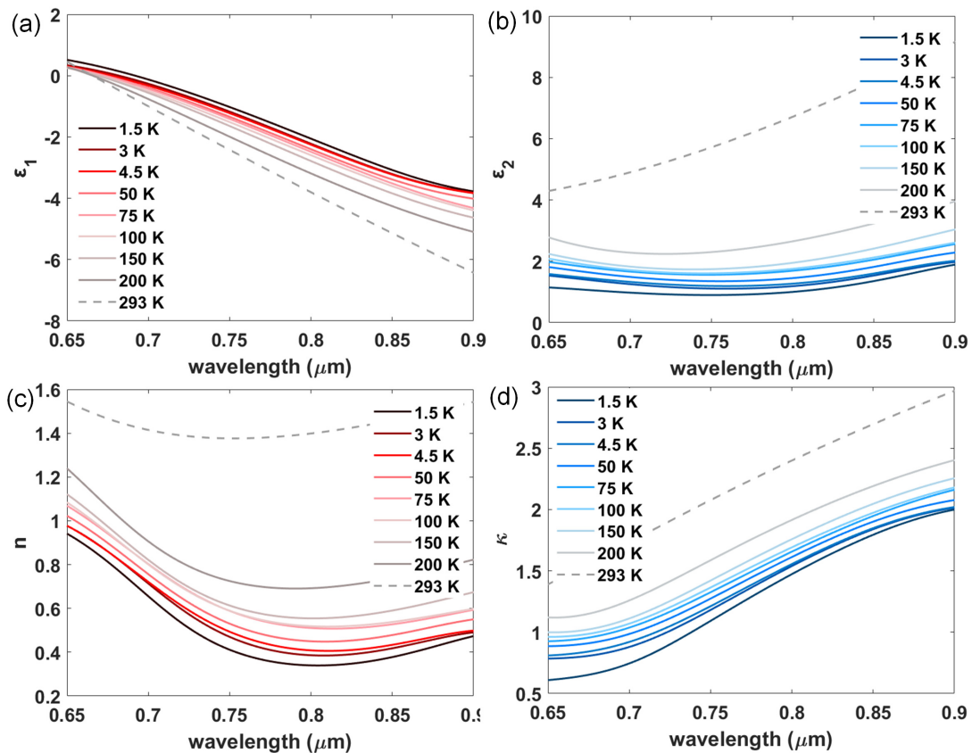
Fig. 2. Real (a,c) and imaginary (b,d) parts of the permittivity ( \epsilon = \epsilon_1 + i\epsilon_2 ) and refractive index ( N = n + i\kappa ), respectively, for a 100 nm TiN film for different temperatures, as a function of the wavelength. The color coding is depicted in the legends.
