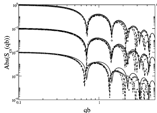
FIG. 4. Chain-core scattering when varying the number of chains for the simulations shown in Fig. 1. The medium and high surface coverage curves have been shifted down two and four decades, respectively. Curves are simulation results without excluded volume interactions (full), model 1 (dash-dotted) and model 2 (dashed) fits.
