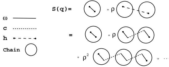
Figure 4.3: Diagrammatic expansion of the PRISM equation in terms of intra-chain correlations \omega(q) , and direct correlation function c(q) .
