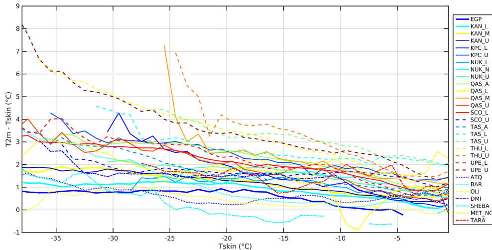
Figure 14. Mean 2 m air temperature and skin temperature differences ( T_{2m} - T_{skin} ) for all sites as a function of binned skin temperature ( T_{skin} ). The T_{skin} bin size is 1 °C, the T_{2m} - T_{skin} bin size is 1 °C and only bins with more than 50 members are considered. Each surface type has its own line style or line width.
