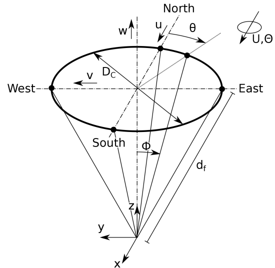
Figure 1. Lidar geometry definitions and coordinate system.
