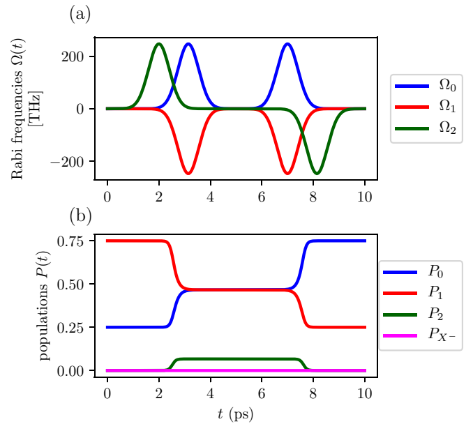
FIG. 6. The time evolution of (a) the laser fields and (b) the populations in a single-qubit NOT operation around the x axis. The initial state is |i\rangle = 0.5 |0\rangle + 0.866 |1\rangle and the parameters used in this calculation are \tau = 0.57 ps, \Delta T = 1.14 ps, \Delta = 0 , \delta_1 = \delta_2 = 0 , \chi = -\pi/4 , \eta = 0 , \zeta = 0 ( \zeta = \pi ) for the first (second) STIRAP, \gamma_{PD} = \gamma_{SD} = \gamma_{SE} = 2 GHz and the peak amplitudes of \Omega_0 , \Omega_1 , and \Omega_2 are 247 THz.
