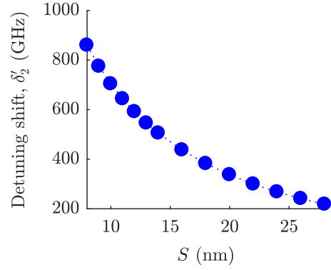
FIG. 9. Shift in two-photon detuning \delta'_2 in DQD_t as a function of the separation, S , between DQD_c and DQD_t after step 1 for a control qubit initially in the state |1\rangle_c .
