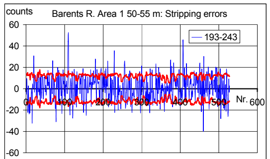
Figure 17. Cobalt window. A1, 50-55m Stripped counts and 2\sigma -intervals".
