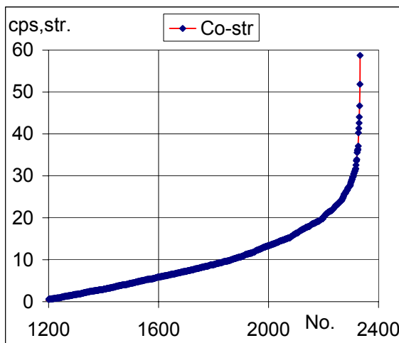
Figure 32. Sorted error plot (positive half) of the stripping errors for the 60 Co window for 30-80m survey height in Area A2. Stripping factors from Area A1 55-60m.
