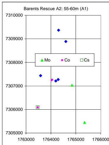
A2. 99m Tc window.
