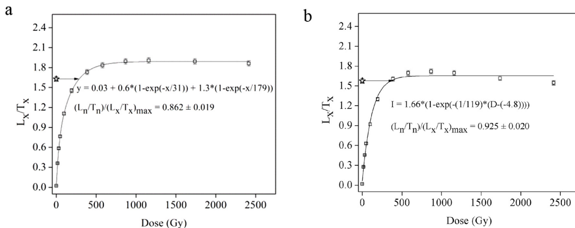
Fig. 3. Synthetic dose response curve constructed using a) the summed OSL signals from 6 multi-grain aliquots and b) the summed OSL signals from 3,800 individual grains of quartz. Data are fitted using a) a sum of two single-saturating exponential functions and b) a single saturating exponential model.
