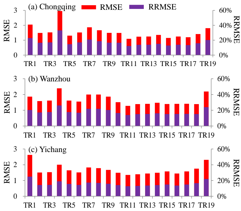
Fig.10 RMSE (MJ m -2 ) and RRMSE of the temperature - relative humidity (TR) models
