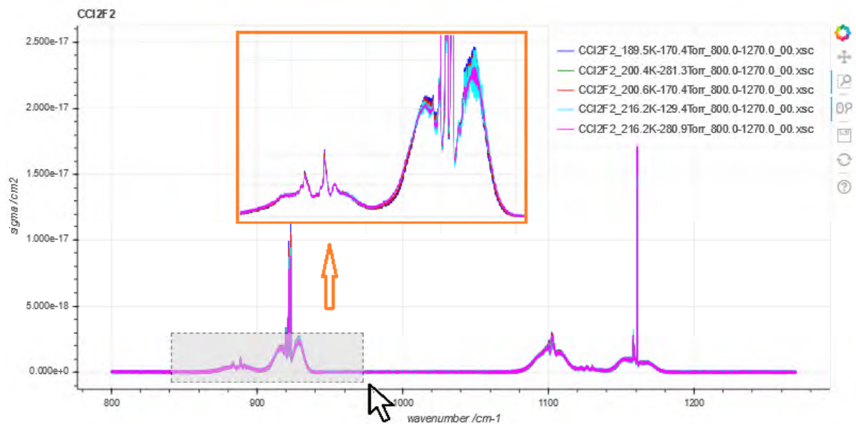
1 2 Figure 28. Interactive spectra view.
