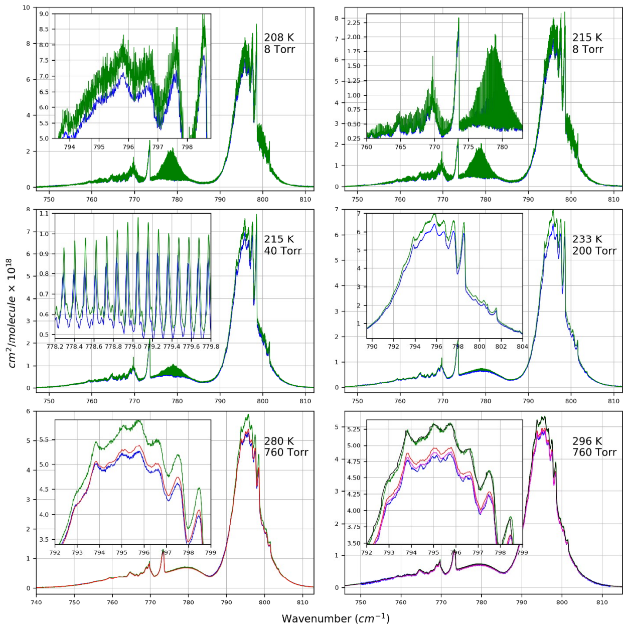
4 5 Figure 15 . Absorption cross-section comparisons for carbon tetrachloride (CCl 4 ). Each panel 6 corresponds to the approximate values of temperature and pressure. Considered spectra: Harrison 7 et al. [28] (green), Varanasi private communication (blue), PNNL [13] (red), NIST [17] (black), 8 Wallington et al. [113] (magenta).
