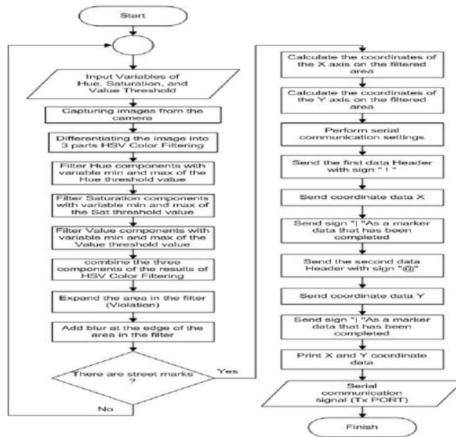
Figure 2. Flowchart of street mark detection system
