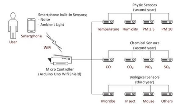
Fig. 5. External Sensors Diagram
