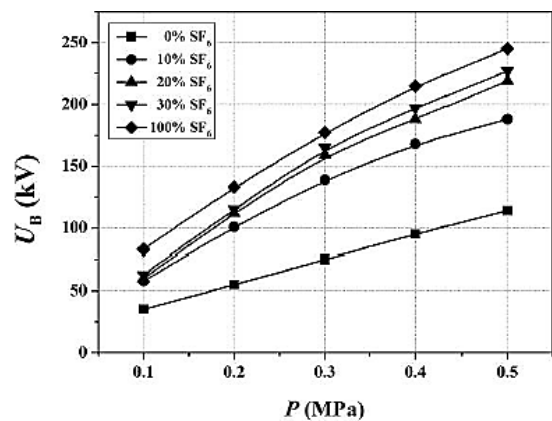
Fig. 1. AC Breakdown voltage of SF 6 /N 2 as a function of gas pressure under R8-plane configurations [8].
