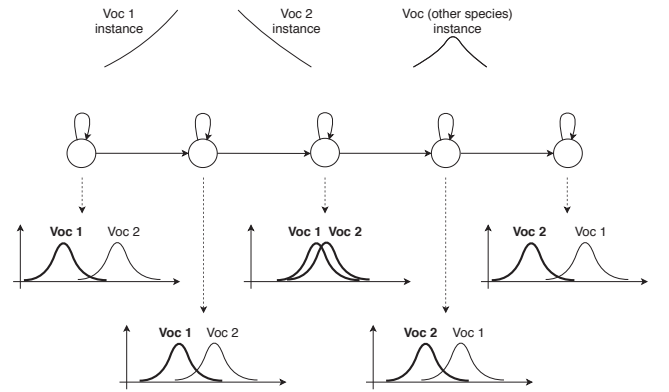
Fig. 3. An illustration of the drawback of using a single HMM per bird species, with GMM at each state.
