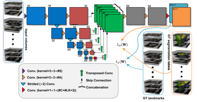
Fig. 4. The architecture of the proposed SSSLN with 15 convolutional layers. The network takes different CMR volumes as input, applies a branch of convolutions, learns image features from fine to coarse levels, concatenates multi-scale features and finally predicts the probability maps of segmentation and landmarks simultaneously. These probability maps, together with the ground-truth segmentation labels and landmark locations, are then utilized in the loss function in (1) which is minimized via the stochastic gradient descent. Here #S, #A, #C, #LK and GT represent the number of volume slices, the number of activation maps, the number of anatomies, the number of landmarks, and ground truth, respectively.
