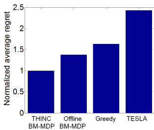
Figure 7: Solution quality
