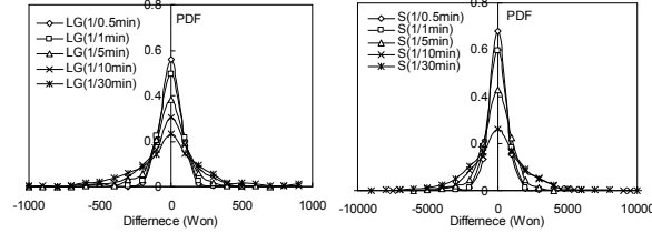
Fig. 22. PDF for difference of two consecutive values in stock prices
