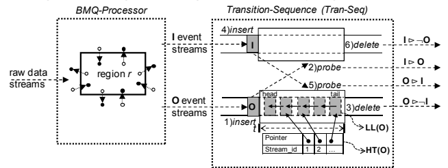
Fig. 7. Processing flow of RTMQ
