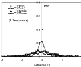
Fig. 25. PDF of difference
