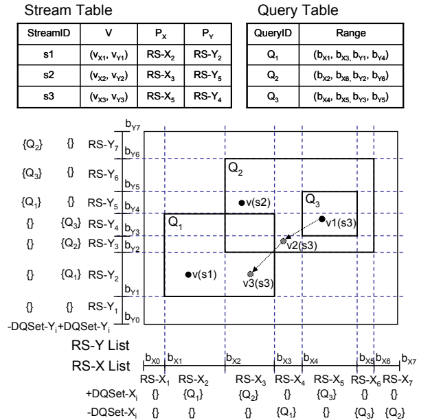
Fig. 4. Two-dimensional BMQ-Processor
