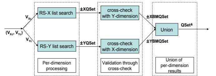
Fig. 4. Two-dimensional BMQ-Processor
