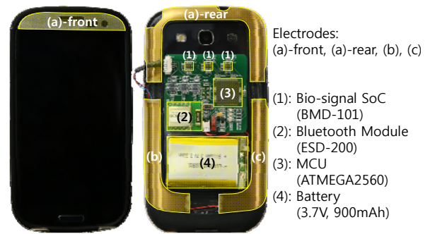
Figure 3. Sinabro sensor
