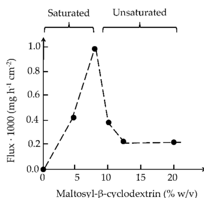
Figure 3. The effect of maltosyl-β-cyclodextrin concentration on the permeation of hydrocortisone through hairless mouse skin in vitro. The amount of hydrocortisone in the aqueous donor medium was kept constant 16 mg/mL but the maltosyl-β-cyclodextrin concentration was from 0 to 20% ( w/v ). Below 8% ( w/v ) maltosyl-β-cyclodextrin the medium was hydrocortisone suspension in water, but hydrocortisone solution in water at higher concentrations. Based on unpublished results.
