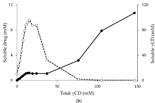
Figure 4. The phase-solubility diagram of hydrocortisone/HP \gamma CD (a) [58] and hydrocortisone/ \gamma CD (b) [59] complex. Concentrations of the soluble drug (open circle) and CD (filled circle) are plotted against the concentration of total CD.
