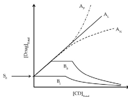
Figure 2. Types of phase-solubility diagrams according to Higuchi and Connors [11] showing how the total drug solubility changes with increasing CD concentration. A-type diagrams are formed when the drug/CD complex is soluble in the aqueous complexation media and they are usually associated with the water-soluble CD derivatives. B-type diagrams are observed when the complex has limited solubility in the media and these are usually associated with the natural CDs that have limited solubility in aqueous media. A_L : linear diagram; A_P : positive deviation from linearity; A_N : negative deviation from linearity; B_S : the complex has some but limited solubility; B_I : the complex is insoluble.
