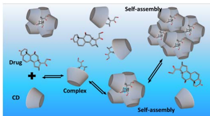
Figure 1. Formation of a cyclodextrin inclusion complex in an aqueous solution and self-assembly of cyclodextrin complexes.
