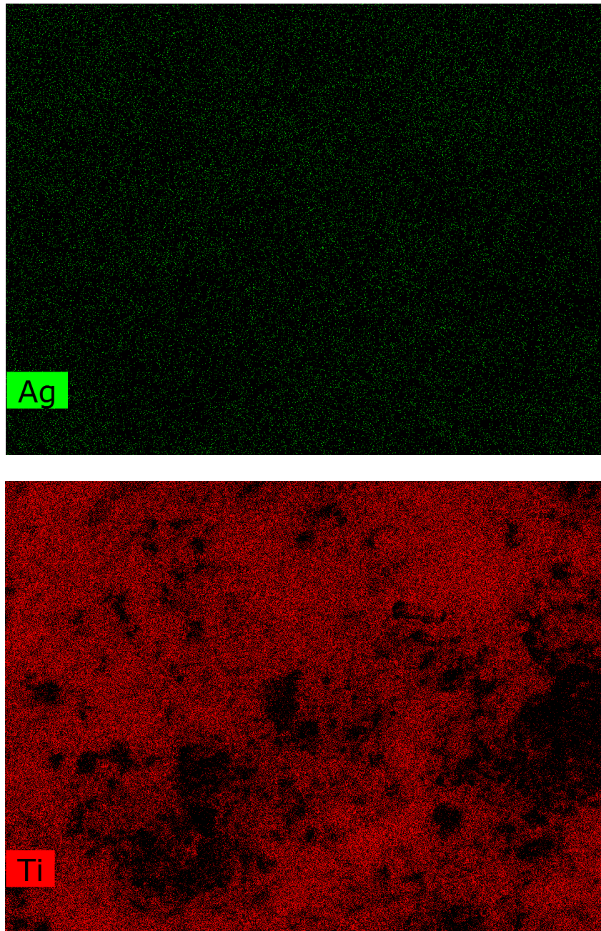
Figure 3 - EDX images of AgNPs-doped micro-sized TiO 2 coated on the ceramic surface obtained after digital printing process. 1) Ag distribution: green spots 2) Ti distribution: red spots
