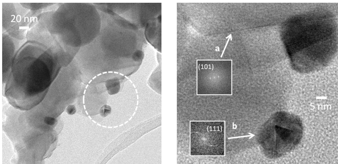
Figure 1b. TEM images of AgNPs-doped TiO 2 . Left-hand section: low magnification image. Right-hand image: high magnification image and electron diffraction patterns.
