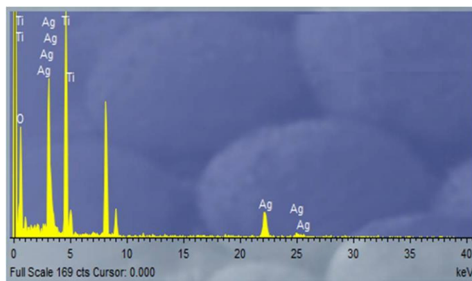
Figure 1c. EDS spectrum relative to the left-hand image reported in figure 1b
