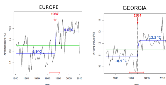
Fig. 1. Change point analysis of average yearly temperature performed for Western Europe and Georgia.
