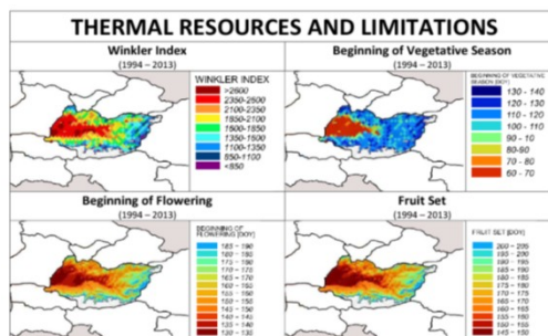
Fig. 3. Imereti region card, thermal resources and limitations.
