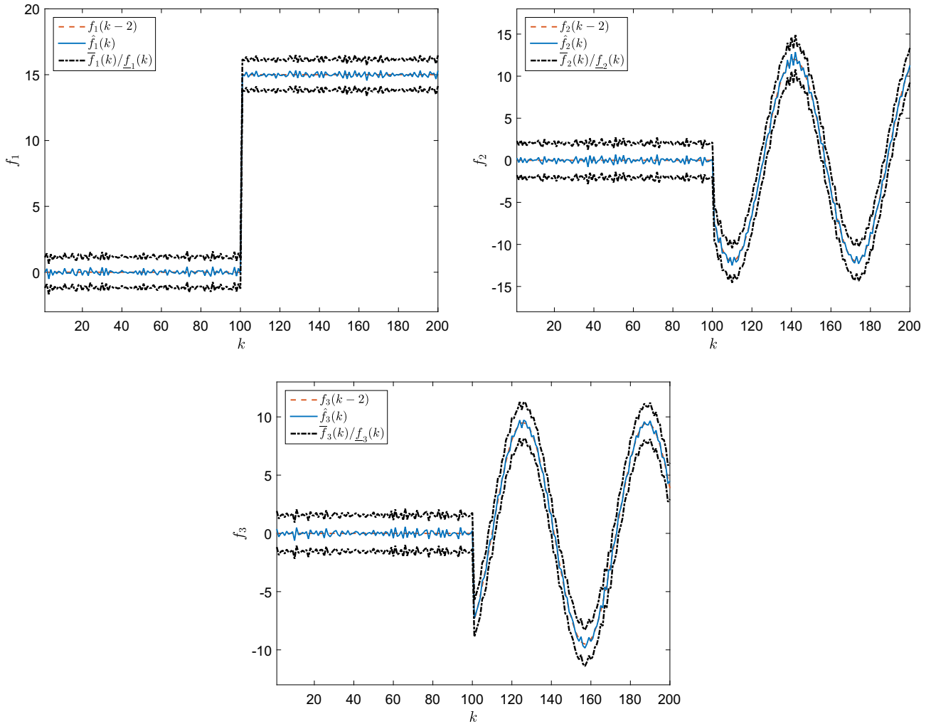
FIGURE 2 The actuator-fault estimation results of the machine infinite bus system [Colour figure can be viewed at wileyonlinelibrary.com ]
