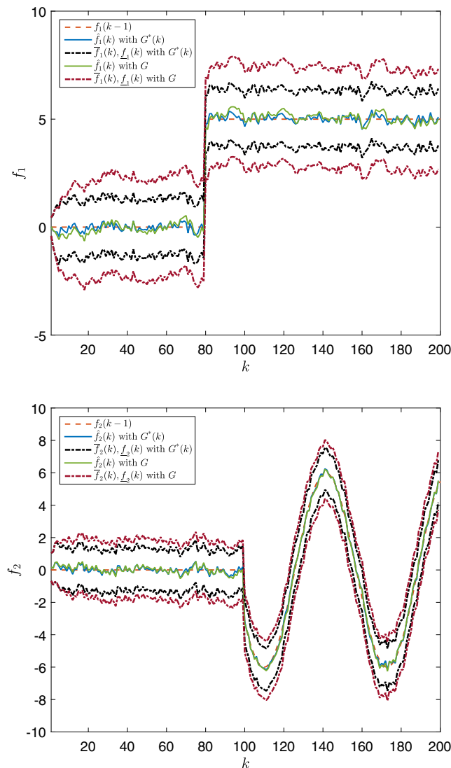
FIGURE 1 The actuator-fault estimation results with G^*(k) and G [Colour figure can be viewed at wileyonlinelibrary.com ]
