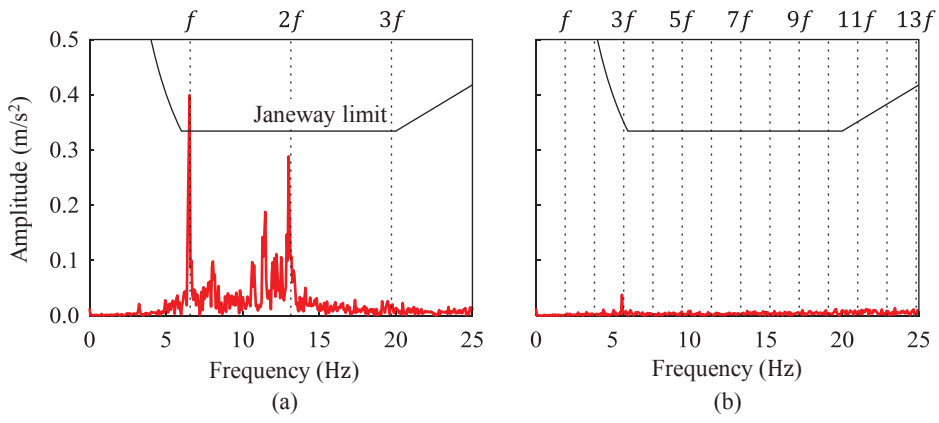
Fig. 19 Measurement results of vertical vibration in vehicle motion: (a) Vibration of the vehicle with the conventional AOW ( f = 6.57 \text{ Hz} ). (b) Vibration of the vehicle with the new AOW ( f = 1.91 \text{ Hz} ). The black line indicates Janeway's recommended amplitude limit [25].
