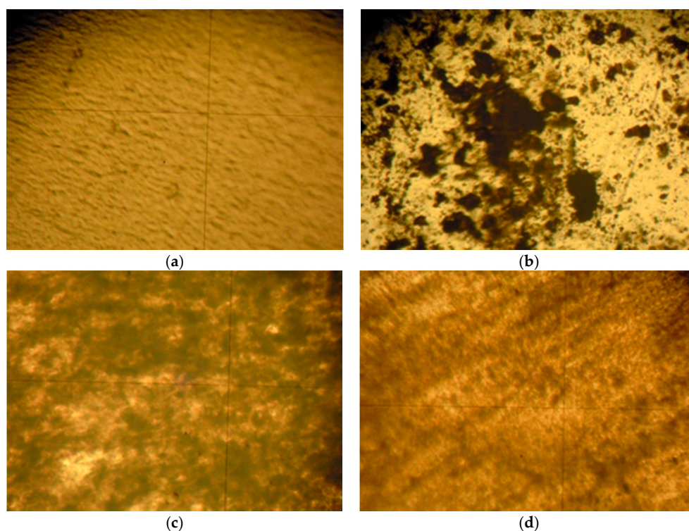
Figure 7. Optical micrographs (100 \times ) of polyethylene films: (a) LDPE; (b) LDPE + 5% \beta CDTiO 2 NPs (mortar grinding); (c) LDPE + 5% TiO 2 NPs (cryo-milled mixture); (d) LDPE + 5% \beta CDTiO 2 NPs (cryo-milled mixture).
