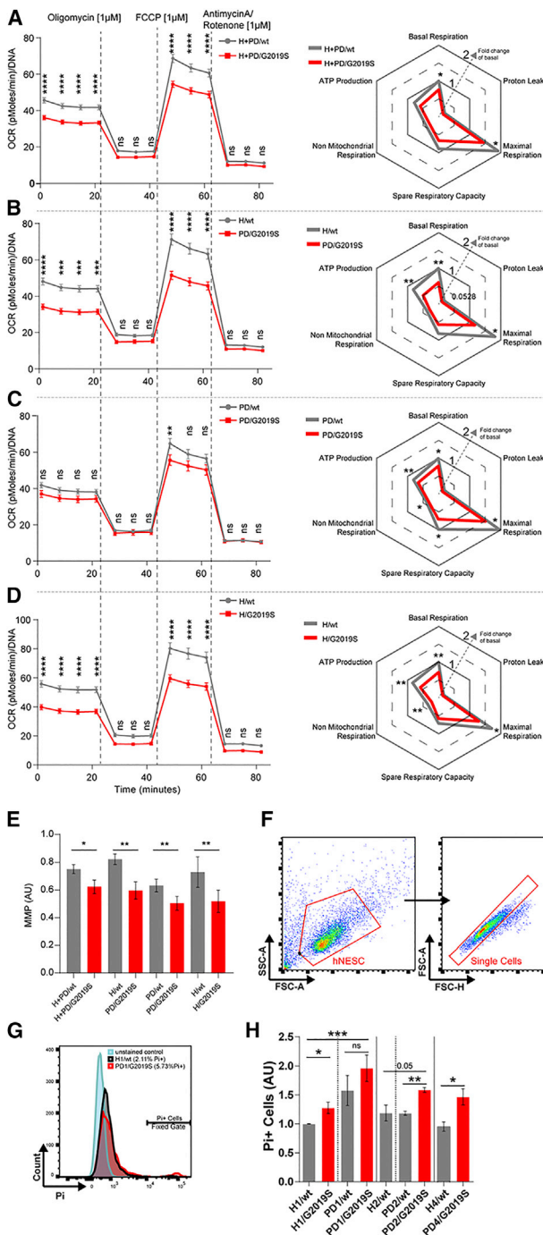
Figure 3. LRRK2-G2019S Induces Loss of Respiratory Capacity and Cell Death
