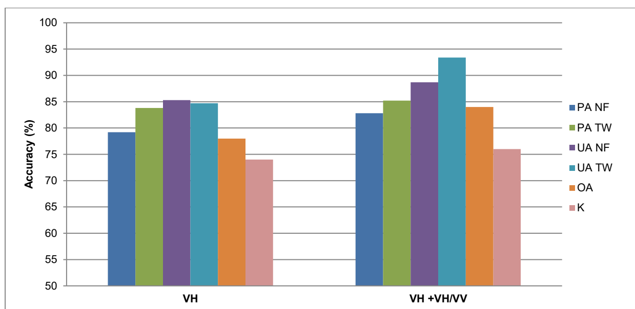
Figure 4.9 Classification accuracy results for the time series approach for VH and fusion of VH and VH/VV images for 6 April 2017
