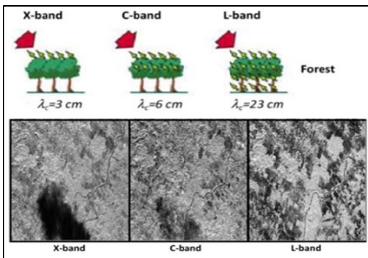
Figure 2.4 Response of a forest stand to X-, C- and L-band microwave energy
