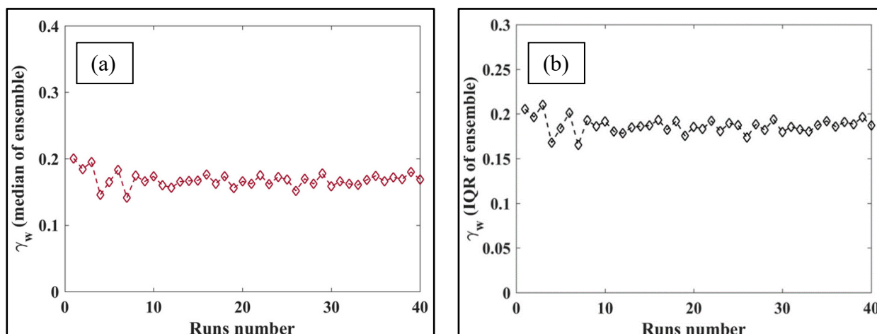
Figure 3.10 (a) Medians; (b) interquartile range (IQR) of ensemble \gamma_w calculated over the study area as a function of number of runs included in the ensemble
