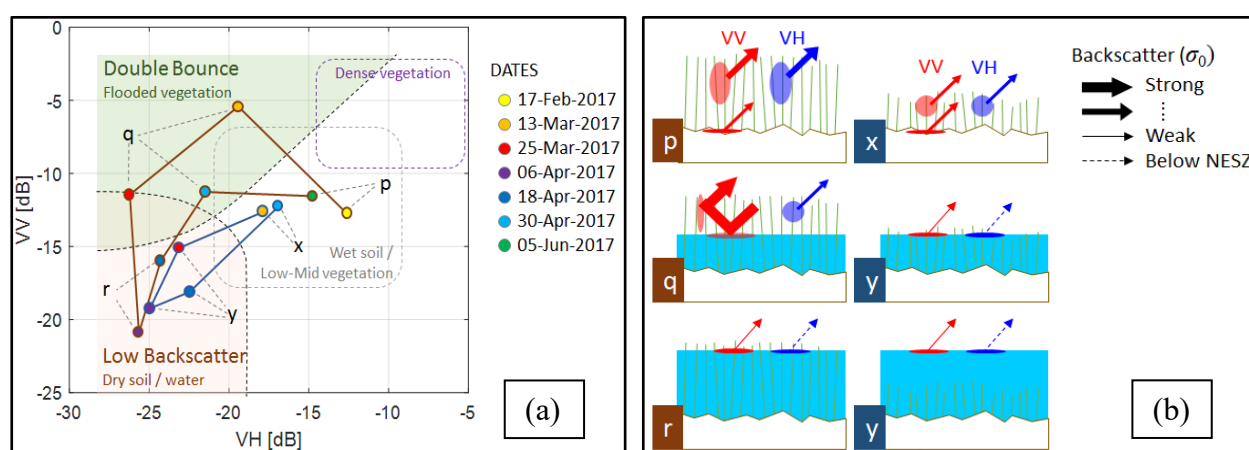
Figure 4.3 The (a) Sentinel-1 time series in the VH and VV plane of two different pixels before, during and after the flood event. The first location (dark red line) has tall grass and shrubs whereas the second (blue line) has short grass. The coloured markers show the temporal information. In the first location, the flooding period started earlier and ended later than in the second location. (b) Schematic representation of the scattering mechanisms for the different LC types and different flood levels. Note: The scenarios r and z essentially produce the same mechanism type and NESZ is the noise equivalent sigma zero
