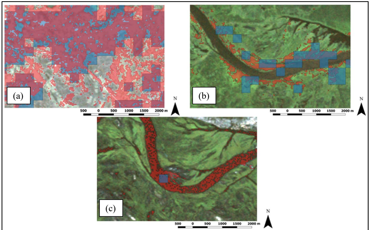
Figure 3.8 Different extents of (a) soil, (b) vegetation and (c) water endmembers selected by the automatic procedure explained in Section 2.6 from TM (red shade) and MERIS images (blue shade) on 17 April 2008 over TM true colour composite (RGB)
