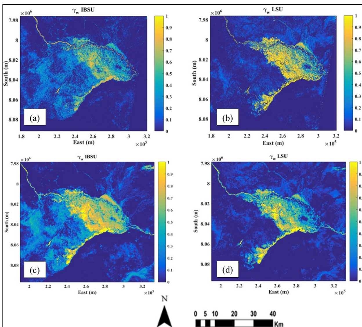
Figure 3.14 The \gamma_w maps produced by applying (a) IBSU and (b) LSU on the 17 April 2008 TM image, compared to (c) IBSU and (d) LSU applied to the MERIS image of the same date
