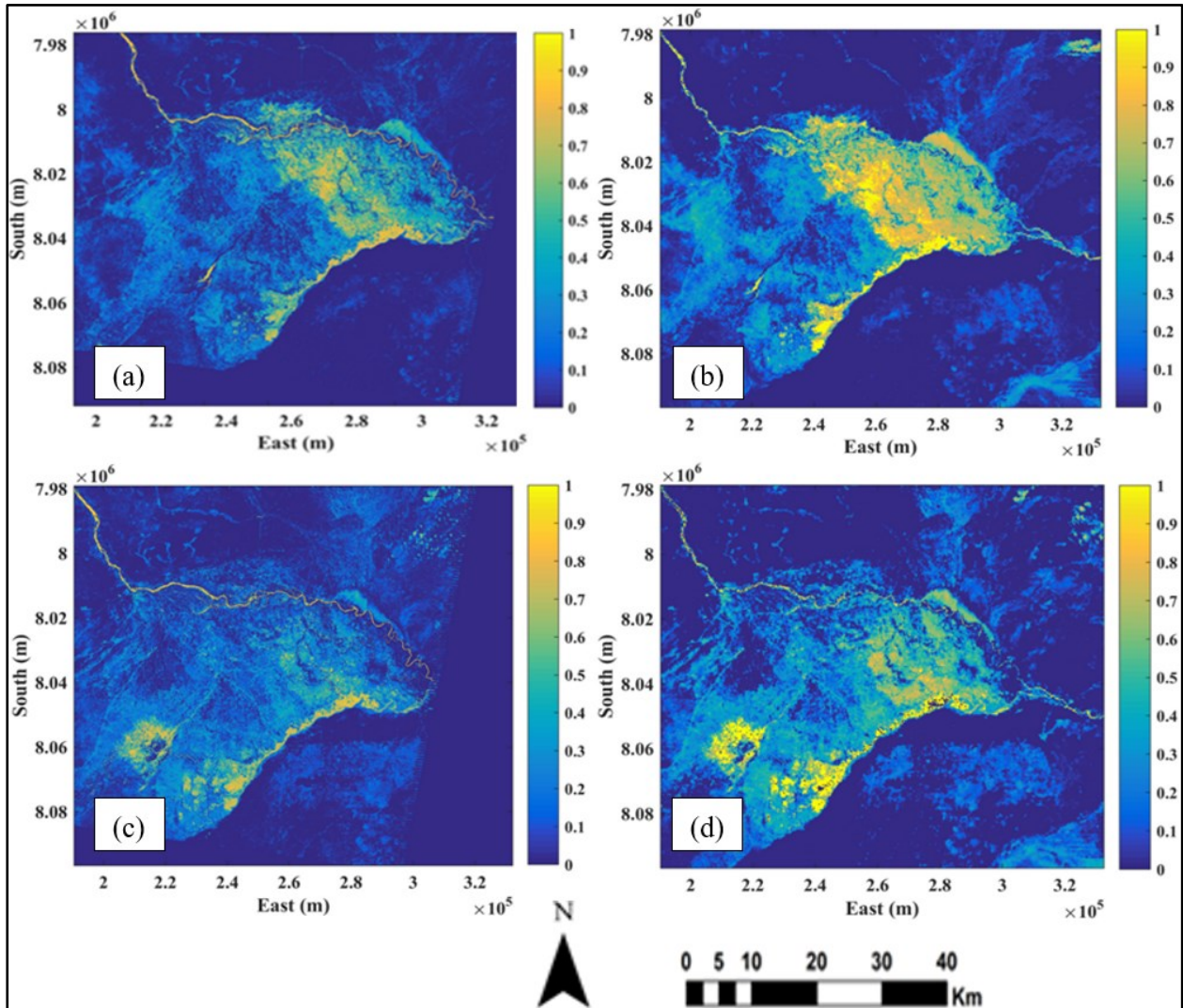
Figure 3.11 The \gamma_w calculated with the 17 April 2008 (a) TM and (b) MERIS images, compared to the \gamma_w derived from the (c) 22 May 2009 and (d) 23 May 2009 MERIS images
