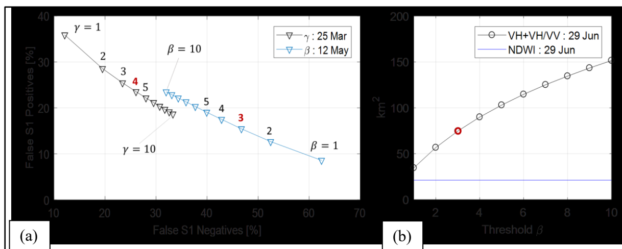
Figure 4.5 The (a) performance of the algorithm for different likelihood ratio thresholds \gamma and \beta evaluated on the LS and S1 images, collected on 25 March 2017 (flood peak) and 12 May 2017 (flood recession) and (b) estimated flooded area by algorithm (VH + VH/VV) and by the LS NDWI thresholding method on the images collected on 29 June 2017. The selected thresholds ( \gamma = 4 and \beta = 3 ) are highlighted
