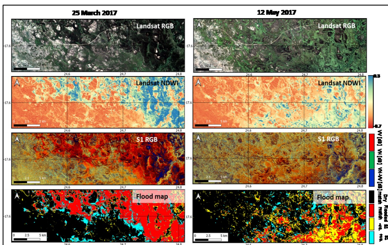
Figure 4.11 Comparison during flood peak (25 March 2017) and recession (12 May 2017) in the area surrounding the Malindi village, with (a) showing an RGB colour composite (3, 2, 1) and (b) an NDWI derived from Landsat. The Sentinel-1 polarisations (VV, VH, VH/VV) are shown as a colour composite (c), while the flood maps generated by the merging (union) of the TW and FV maps are shown in (d). The matching pixels between the NDWI and the merged S1 dataset are depicted in black and red for the dry (non-flooded) and the flooded areas respectively. The (false) S1 negatives and positives are shown with yellow and magenta.
