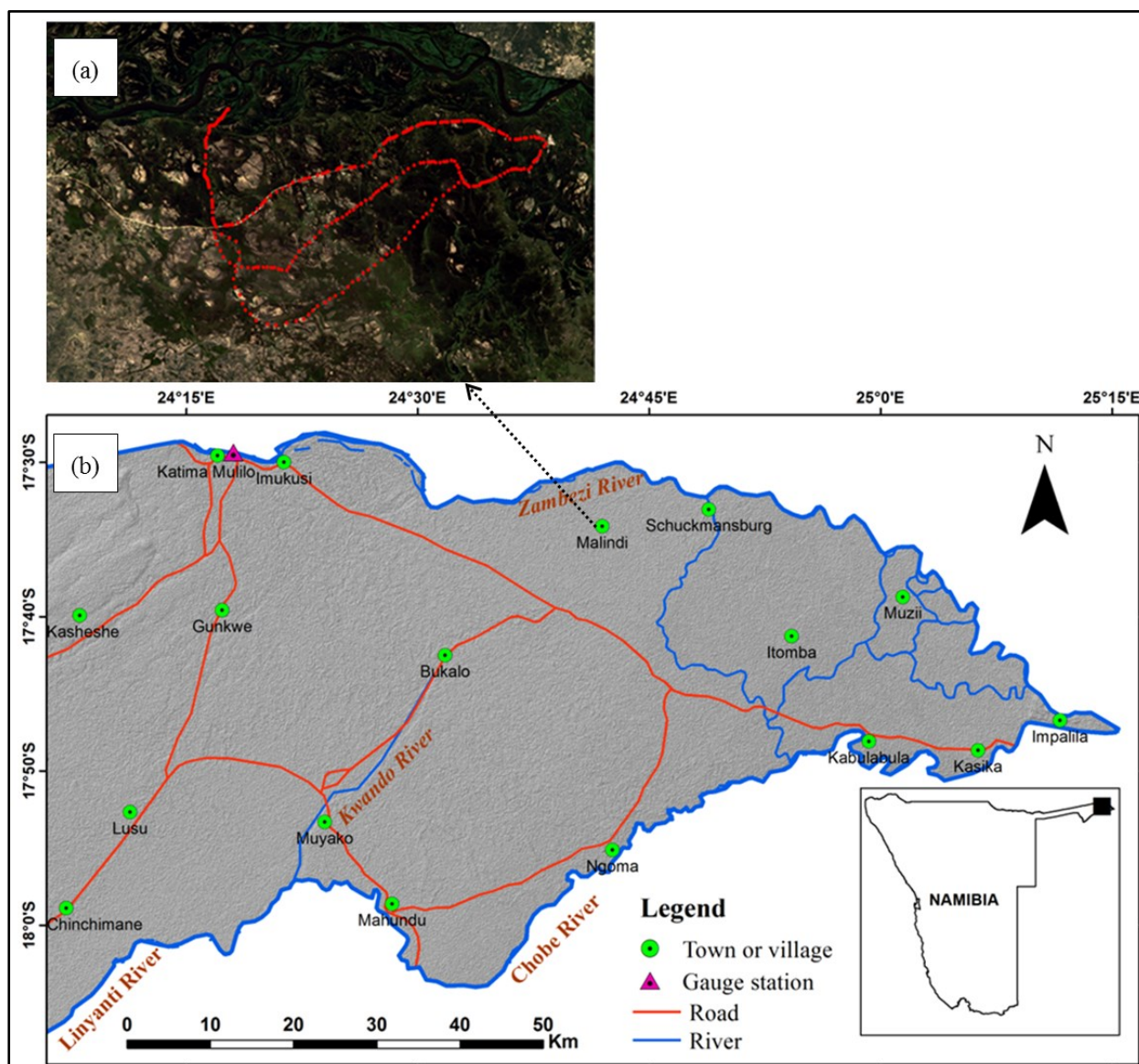
Figure 4.1 Location map of the (a) collected ground observations overlaid on a true colour image (4, 3, 2) of Landsat-8 (10 April 2017) and (b) study area
