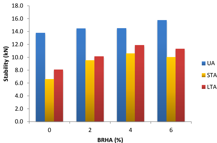
Fig. 2: Stability of asphalt mixtures at different aging conditions
