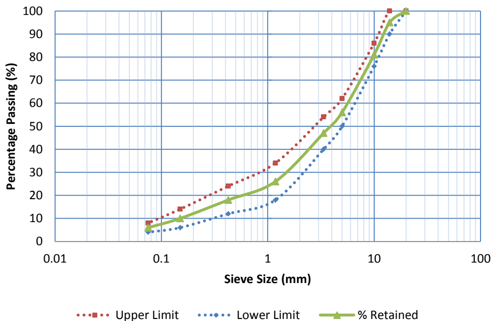
Fig. 1: The aggregates gradation
