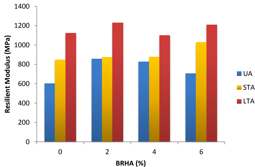
Fig. 4: Resilient modulus of asphalt mixtures at 40°C
