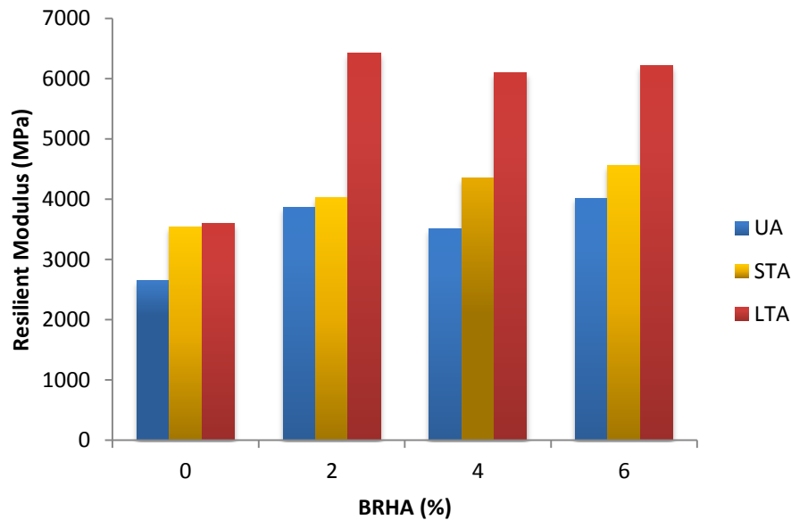
Fig. 3: Resilient modulus of asphalt mixtures at 25°C
