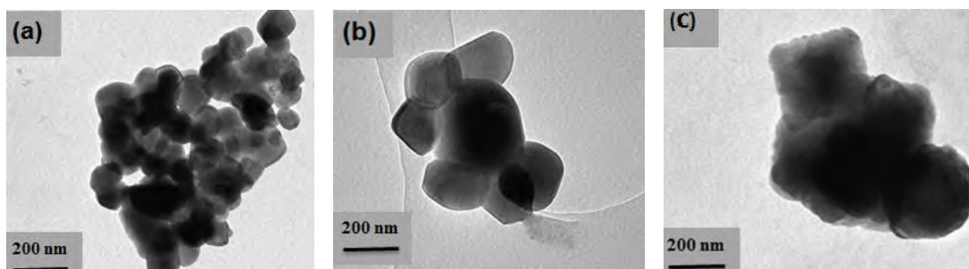
Figure 6: TEM Micrographs of Zn_{0.7}Co_{0.3}MoO_4 treated at 500^\circ C (a) / 700^\circ C (b) and 800^\circ C (c).
