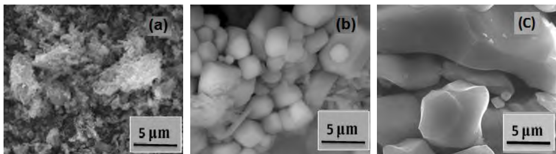
Figure 5: SEM micrograph of Zn_{0.7}Co_{0.3}MoO_4 treated at 500^\circ C (a) / 700^\circ C (b) and 800^\circ C (c).
