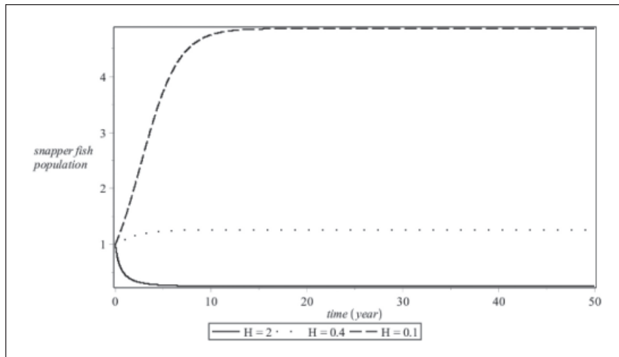
Fig. 4. The dynamics of snapper fish population over time in year for various values of fishing rate H . The solid line shows for H = 2 , the dotted line shows for H = 0.4 and the dashed line shows for H = 0.1 .
