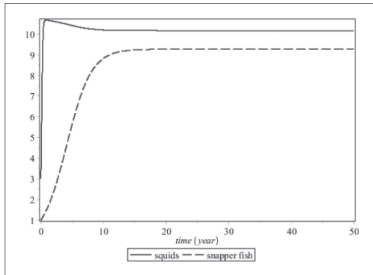
Fig. 2. Time series plot for squids and snapper fish where in the future (after 50 years), the populations will stabilize to (x_4, y_4) = (10, 9) with initial population (x_0, y_0) = (3, 1) for the same fishing rate E = H = 0.05 .
