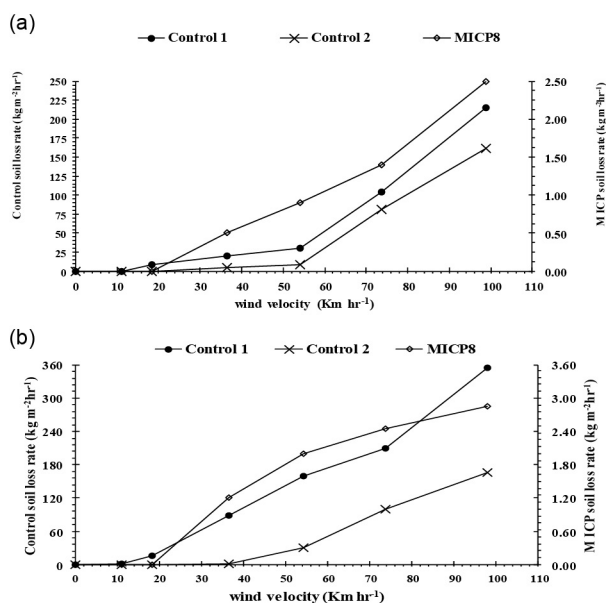
Figure 5. Soil loss rate (kg. m 2 .h -1 ) in sandy loam (a) and silty loam (b) at different velocities in MICP8 treatment.
