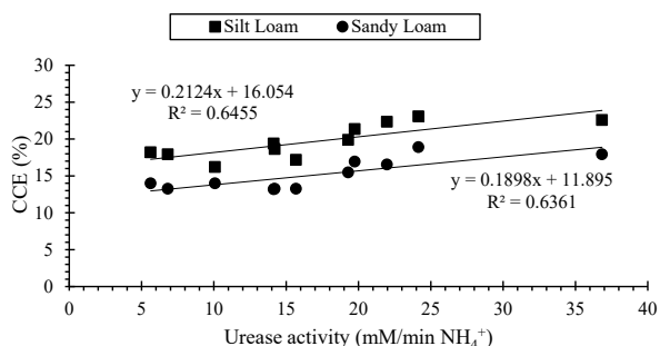
Figure 4. Relationship between calcium carbonate precipitation (%) and urease activity (mM/min NH 4 + ).
