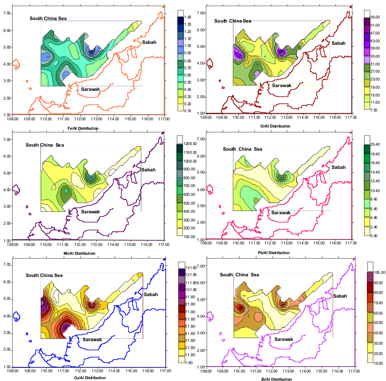
Fig. 4 The pattern of metal:Al ratios in sediment in the pre-monsoon period.
