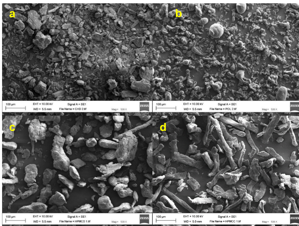
Figure 2 SEM images of (a) CHD (b) P407, (c) HPMC and (d) Methocel x500.
