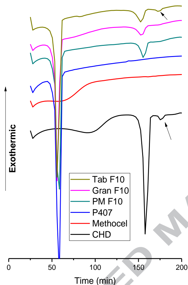
Figure 9 DSC thermograms of F10 physical mix (PM), Granules (GRAN), tablet (TAB), CHD, Methocel and P407.
