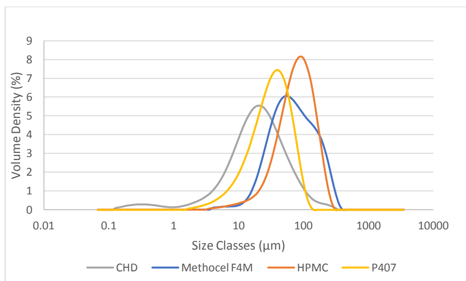
Figure 2 Particle size distribution of CHD, Methocel F4M, HPMC and P407.
