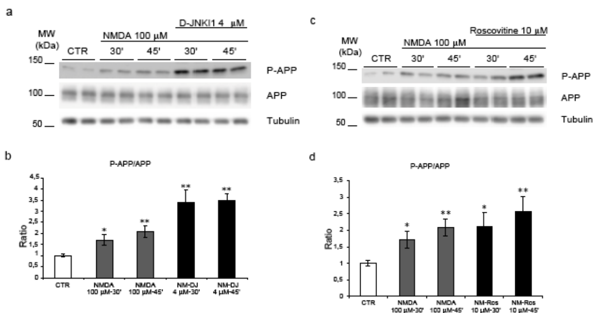
Figure 5. JNK and Cdk5 inhibition do not reverse NMDA induced APP hyperphosphorylation. (a) Neurons were pre-treated with D-JNKI1 and then exposed to NMDA (30'-45'). (b) Western blot analysis and quantification showed that co-treatment with D-JNKI1/NMDA did not reduce P-APP increment induced by NMDA alone. On the contrary, D-JNKI1 pre-treatment increased P-APP/APP level. (NM = NMDA, DJ = D-JNKI1) (c) Neurons were pre-treated with Roscovitine and then exposed to NMDA. (d) Roscovitine did not reduce P-APP following NMDA application. Roscovitine/NMDA co-treatment further increased P-APP/APP levels compared to controls. (Ros = Roscovitine) Loading control: Tubulin. Quantifications are from six independent experiments ( \pm S.E.M.), * p < 0.05 , ** p < 0.01 .
