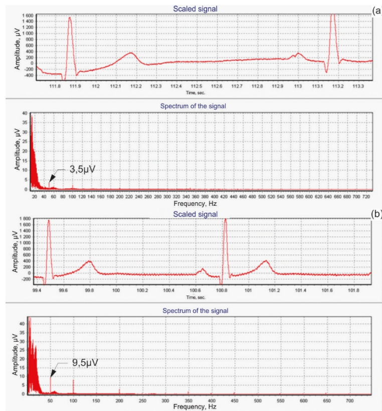
Figure 1. Comparison of electromagnetic pickups of (a) the nanosensor (sensitivity 200 \mu\text{V}/\text{div} ) and (b) the conventional AgCl electrodes by FIAB Spa (Florence, Italy) (sensitivity 200 \mu\text{V}/\text{div} ).
