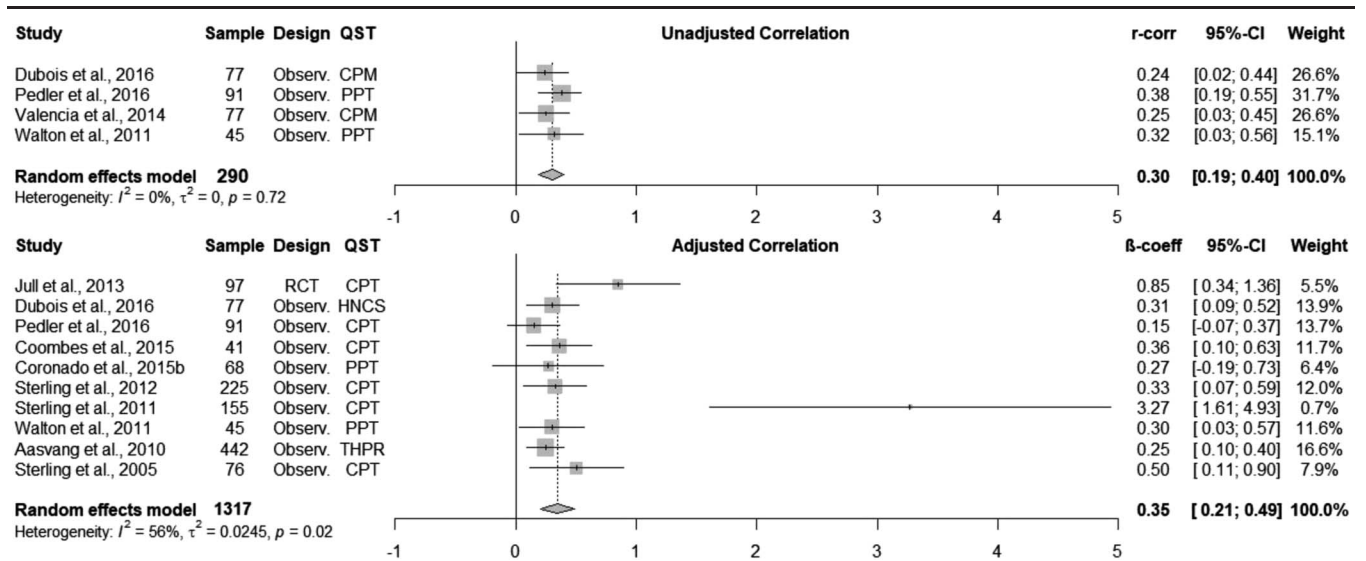
Figure 4. Forest plot showing the overall association (r-correlations and β-coefficients) between QST and follow-up disability in musculoskeletal conditions. CI, confidence interval; CPM, conditioned pain modulation; CPT, cold pain detection threshold; EPT, electrical pain threshold; HNCS, heterotopic noxious counterstimulation; Observ., observational cohort study; PPT, pain pressure threshold; QST, quantitative sensory testing; RCT, randomised controlled trial; THPR, tonic heat pain response. Forest plot showing the pooled unadjusted (0.30, 95% CI: 0.19-0.40) and adjusted correlation (0.35, 95% CI: 0.21-0.49) of QST modalities with musculoskeletal disability. The unadjusted correlation plot has been derived through the incorporation of correlation-coefficient data (Pearson's or Spearman's r) expressing a univariate association unadjusted by other factors, whereas the adjusted correlation plot has been derived through the incorporation of β-coefficient data from linear or logistic regressions expressing a multivariate association.
