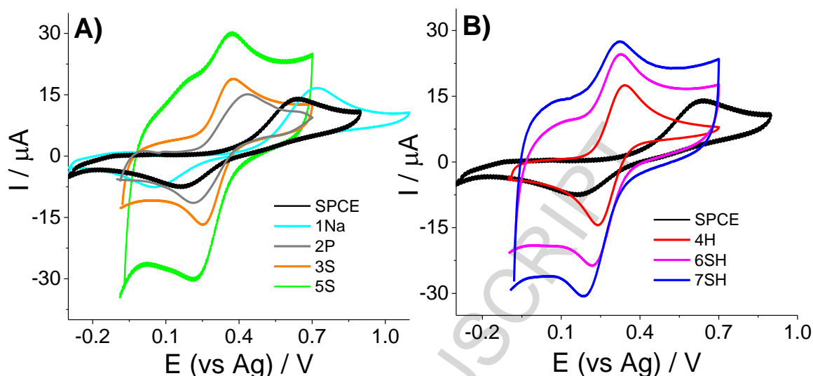
Figure 4. Cyclic voltammetric responses to 1 mM ammonium iron (II) sulfate (in 0.2 M \text{HClO}_4 ) using the nSPCE and aSPCEs obtained after different activation pretreatments. Scan rate: 50 \text{ mVs}^{-1} .
