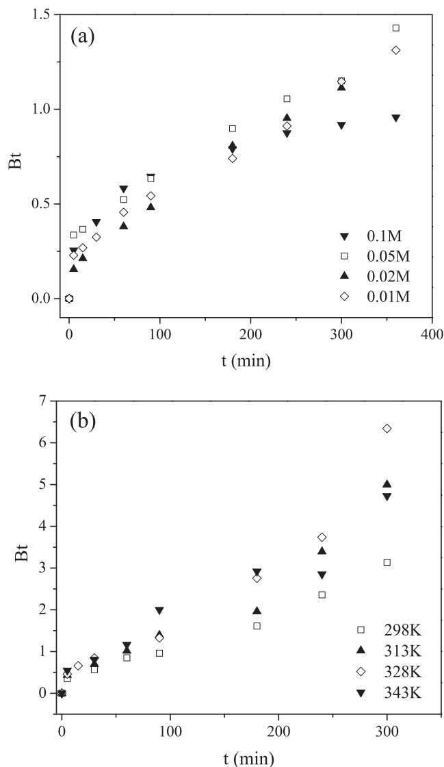
Figure 7 Boyd plots for Mo(VI) sorption by PGME-deta at pH = 2 for: (a) different initial concentrations at 298 K, t = 24 h and (b) different temperatures, C_i = 0.1 M, t = 360 min.
