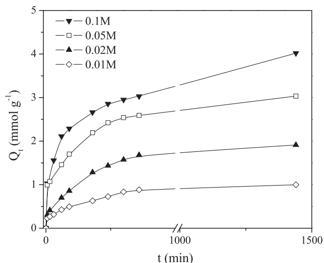
Figure 2 Effect of contact time on the sorption of Mo(VI) on PGME-deta at different initial concentrations ( pH = 2.0 , T = 298 K).
