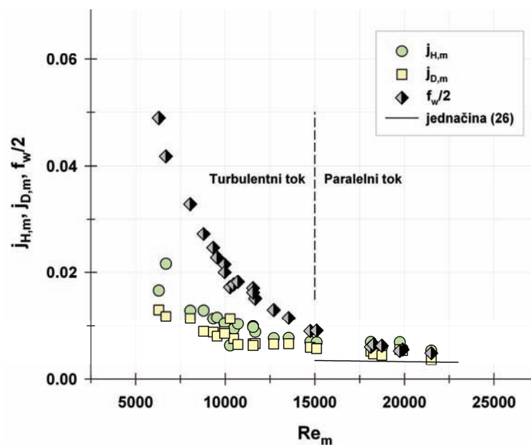
Slika 8. Analogija prenosa količine kretanja, toplote i mase u vertikalnom toku pseudofluida. Figure 8. Analogy among momentum, heat and mass transfer, in vertical flow of pseudofluid.
