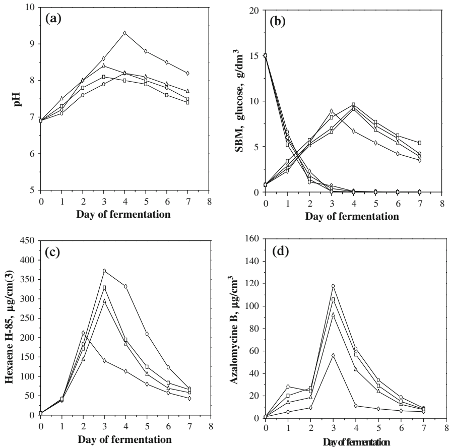
Fig. 2 Change of pH (a), concentration of glucose and dry biomass (b), concentration of Hexaene H-85 (c), and Azalomycine B (d) in basal medium ( \diamond ) and media with Schiff bases: ITC ( \circ ), ISC ( \Delta ), and IPH ( \square )
