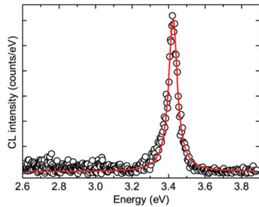
Figure 4. Typical cathodoluminescence spectrum from the GaN:Si thin film showing the experimentally acquired spectrum (circles) and the Voigt fit (line).
