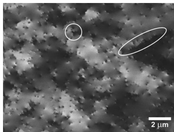
Figure 2. Typical electron channeling contrast image showing threading dislocations (TDs) and tilt/twist across the sample. The white ellipse highlights a line of TDs and the circle highlights a group of closely spaced TDs.
