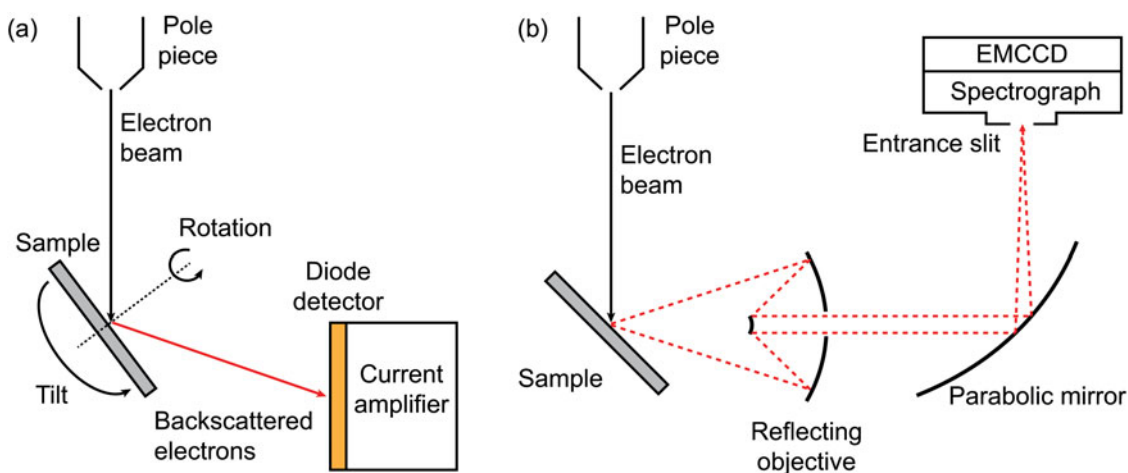
Figure 1. Schematics of the (a) electron channeling contrast imaging and (b) cathodoluminescence experimental setups.
