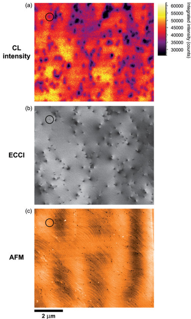
Figure 3. (a) Cathodoluminescence intensity map, (b) electron channeling contrast image, and (c) atomic force microscopy image of the GaN:Si thin film. The feature highlighted by the black circle is probably an inclined dislocation.
