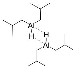
Figure 17 Diisobutylaluminum hydride (DIBAL) as a bridged dimer
