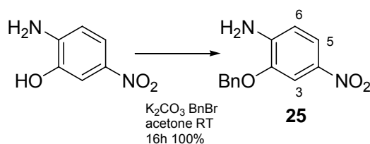
Scheme 74 Benzylation of 2-amino-5-nitro-phenol to form 25
