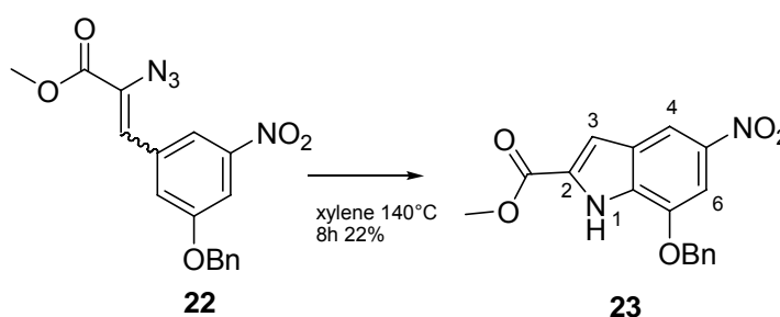
Scheme 71 Hemetsberger indole cyclisation to form 23
