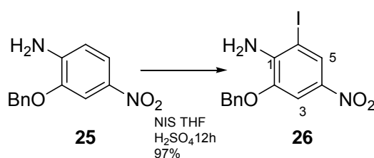
Scheme 75 Iodination at C-3 to form 26
