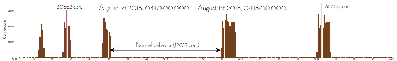
Fig. 5. Time distribution of traffic bursts for the anomaly.
