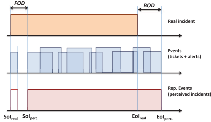
Figure 7: Potential effects of FOD and BOD on the correlation results.
