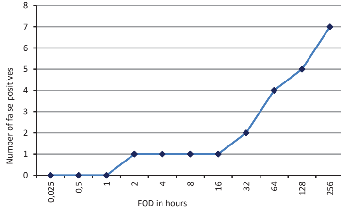
Figure 10: Number of incorrectly correlated incidents (false positives) for different values of FOD.
