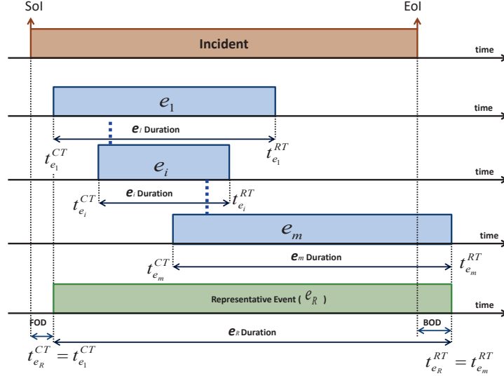
Figure 1: Correlation of m events belonging to the same incident into a representative event.
