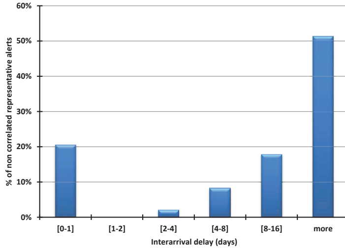
Figure 13: Interarrival delay between consecutive non correlated alerts having the same affected element.
