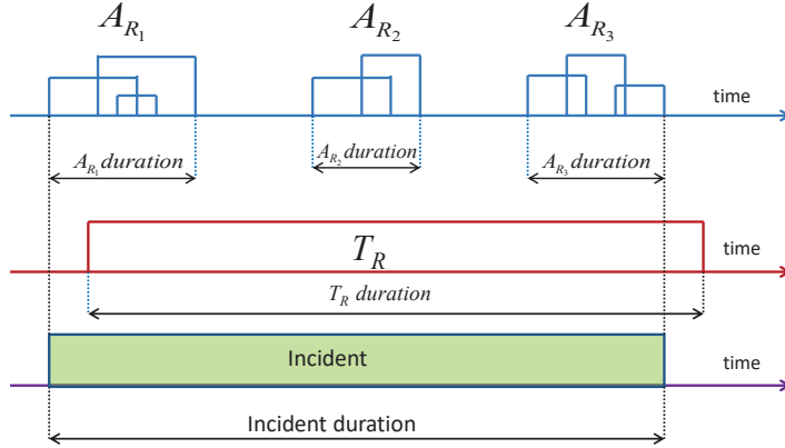
Figure 3: Example of alert aggregation using the proposed model.
