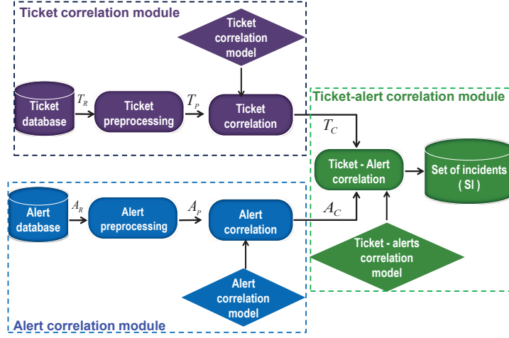
Figure 2: Proposed architecture for the ticket-alert correlation system.
