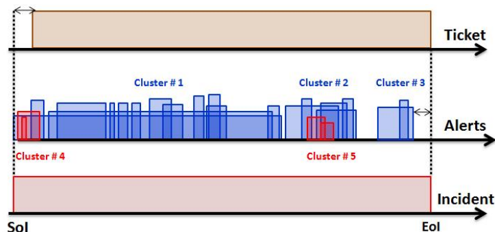
Figure 6: A graphical time representation of the alerts, the ticket, and the generated incident.
