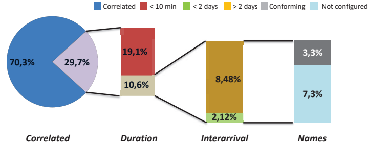
Figure 14: Distribution of the number of raw alerts among the different assessment criteria.
