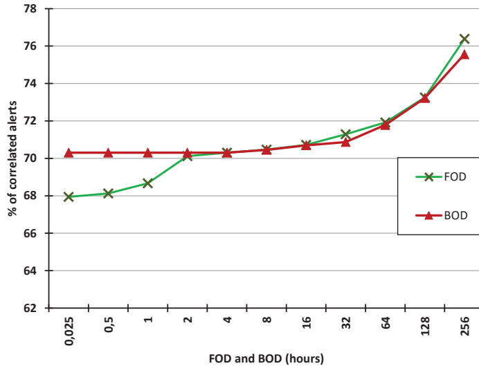
Figure 11: Percentage of correlated alerts at different values for FOD and BOD.
