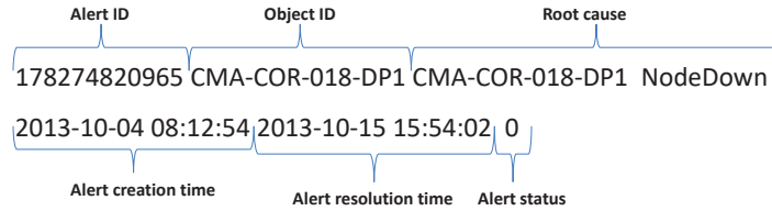
Figure 9: Example of an alert format taken from the alert dataset.
