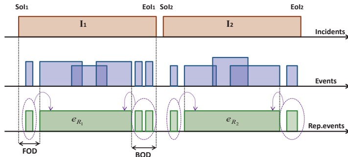
Figure 8: Example showing the problem of directly applying the basic event correlation model to two consecutive incidents.
