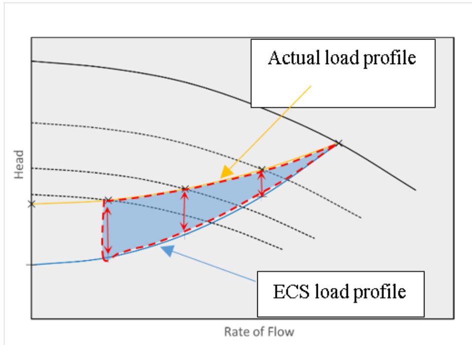
Figure 9. PEI_{VL} Rated Pump Applied in System with Different System Curve than DOE Assumed Load Profile Curve
