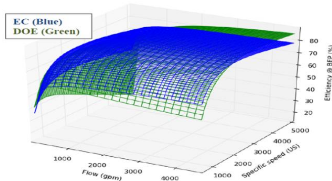
Figure 2. \eta_{\text{pump,std}} Three-dimensional Surface, DOE Compared to EU
