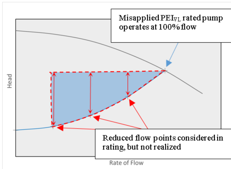
Figure 8. \text{PEI}_{\text{VL}} Rated Pump Applied in Constant Load Application
