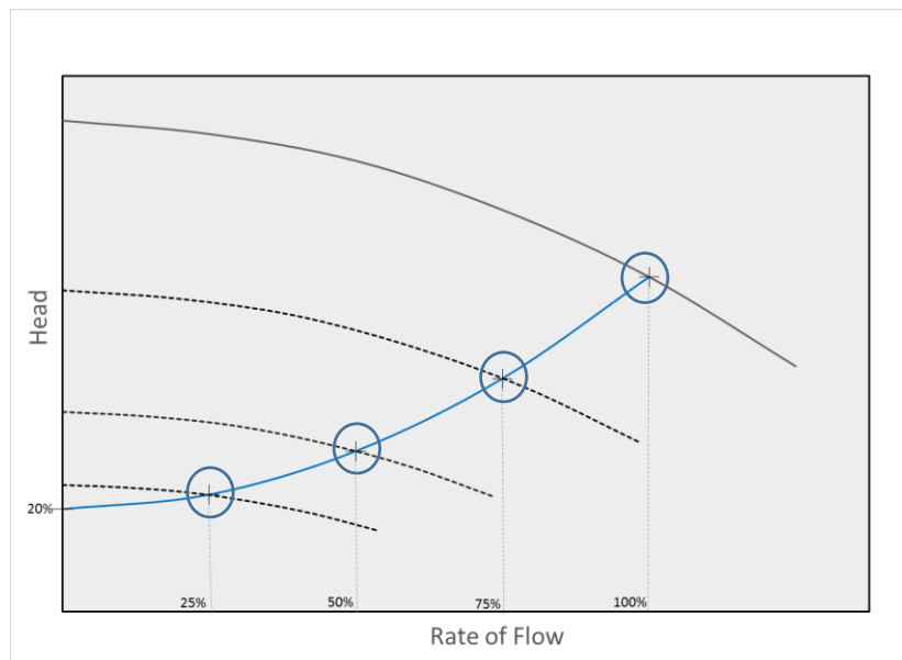
Figure 6. Graphical Representation of Measurements and Continuous Control Standard Load Points to Determine PER_{VL}
