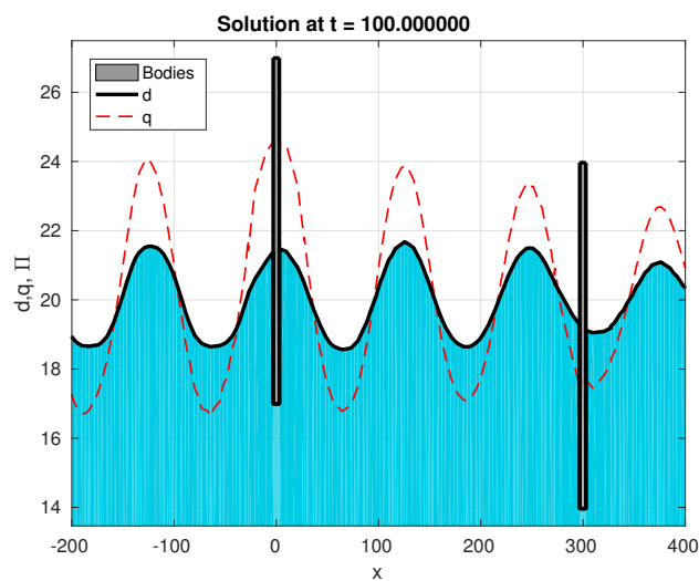
Figure 18: Multi body problem. Each body can be either a fixed pontoon or a heaving body. In figure a the initial set up and in figure b the simulation of two heaving bodies with a wave of period T = 10s and steepness \sigma = 0.025
