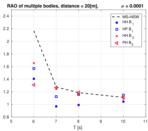
Figure 19: RAO plots for a stream wave of period T = [6, 7, 8, 10]s and steepness \sigma = 0.0001 for the multiple bodies tests with the distance between the bodies dependent on the wave length l = 2\lambda in figure a and for a fixed distance of 20 meters in b: the dashed line is the single body RAO, * and x the first and second heaving bodies in series, □ a heaving body in front of a pontoon and finally ◁, a heaving body behind a pontoon.
