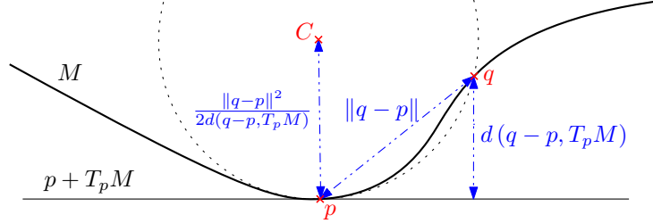
Figure 1: Geometric interpretation of quantities involved in (2.3).
