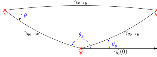
Figure 7: Layout of Lemma 4.5.
