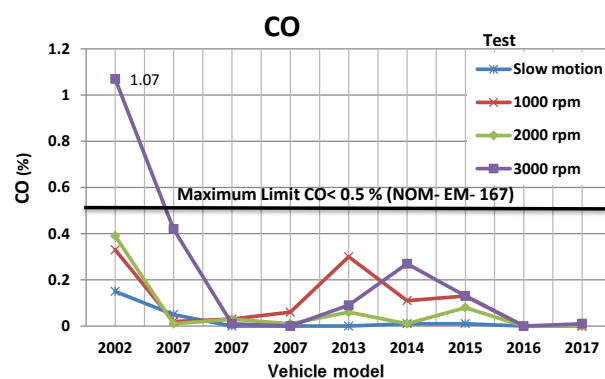
Graphic 2 CO emissions of the vehicles analyzed at different operating conditions Source: Own Elaboration
